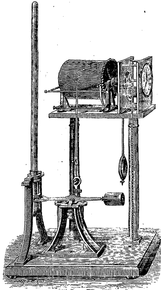
FIG. 2. — Barographe.
