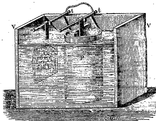
FIG. 2. — Galvanoplastie; appareil simple.
