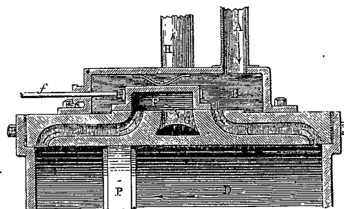
FIG. 5. Tiroir; seconde position.
