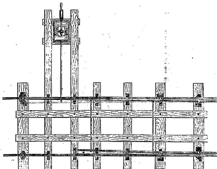
FIG. 4. Aiguilles simples; plan horizontal.
