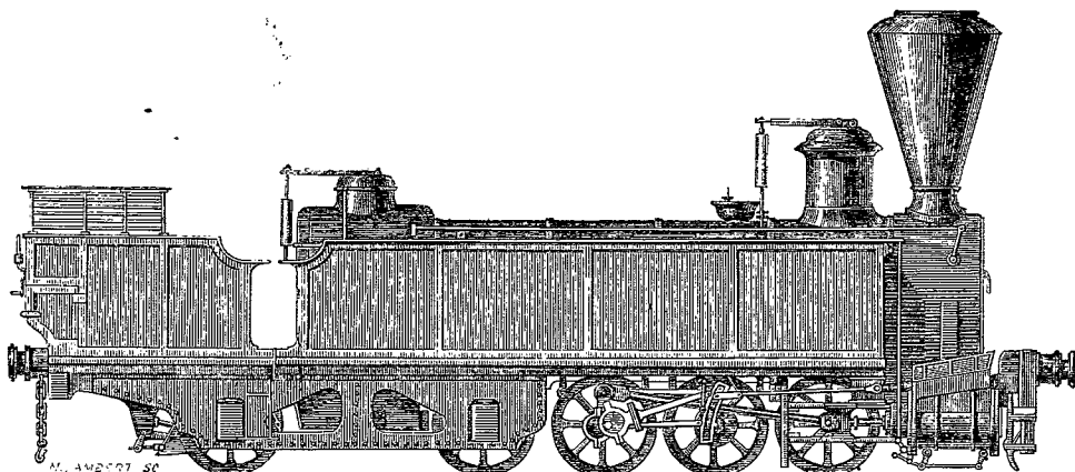
FIG. 7. — Locomotive Engerth.
