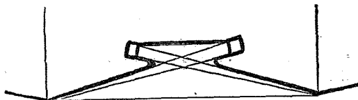
(Fig. 4. — Front de Coehorn.)
